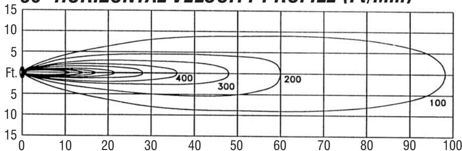
30" HORIZONTAL VELOCITY PROFILE (Ft/Min)
