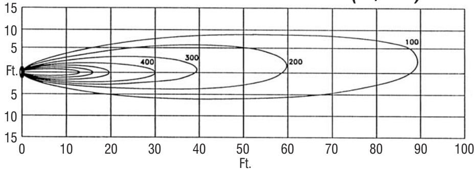
24" HORIZONTAL VELOCITY PROFILE (Ft/Min)
